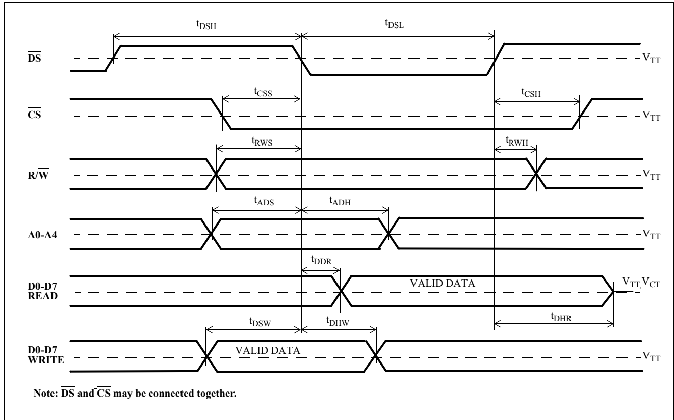
Figure 15 - Microport Timing
